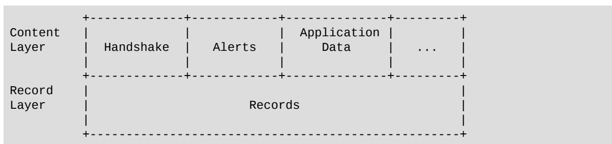
Figure 1: TLS Layers
